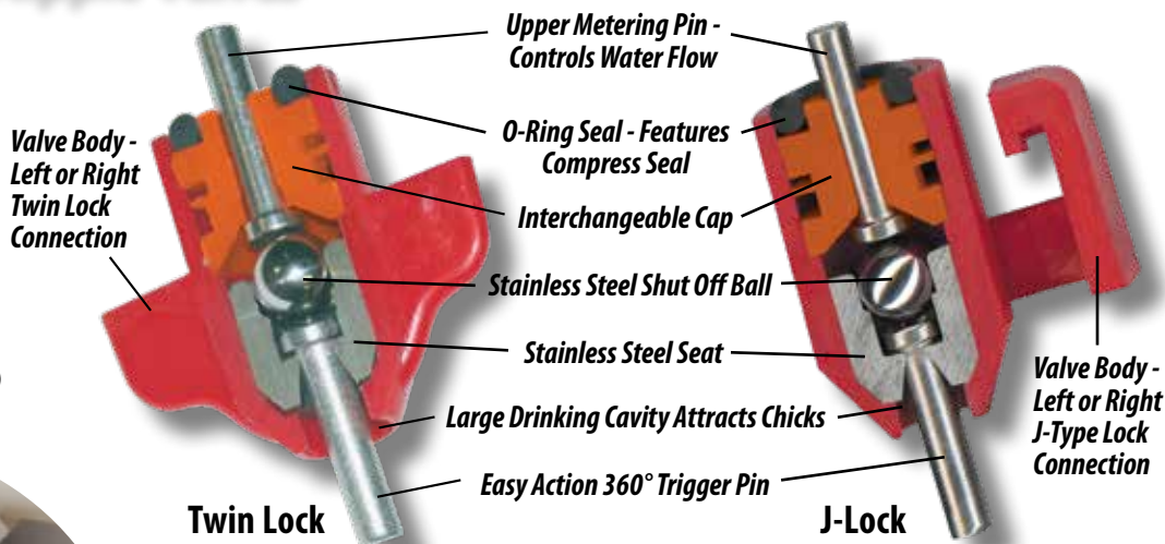
Cumberland's nipple drinker system includes the 360° side-to-side nipple valve toggle action, plus an increased flow rate with vertical lift action.
