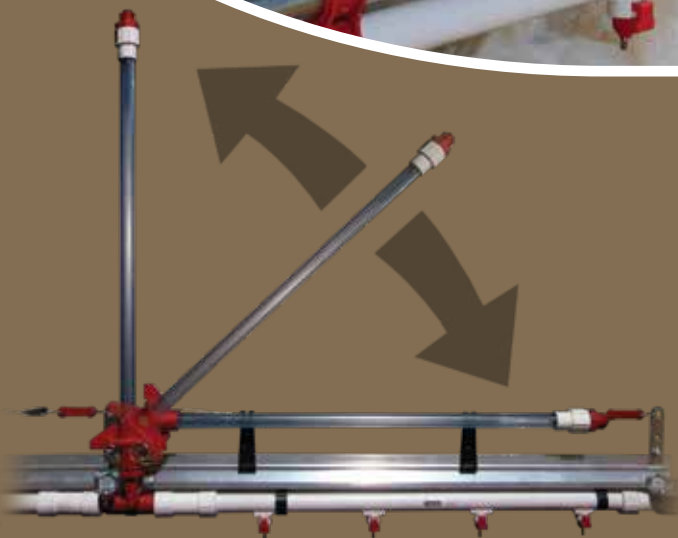
Optional COLLAPSIBLE RIGID STAND PIPE provides unencumbered raising of the watering line.
